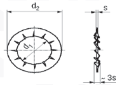
DIN 6798 Type J Internally Toothed
