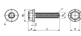
Hex Washer Type D
